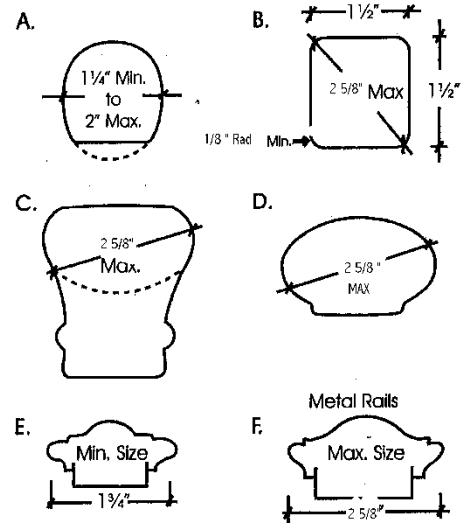
Figure 1014.3 HANDRAIL PROFILES
